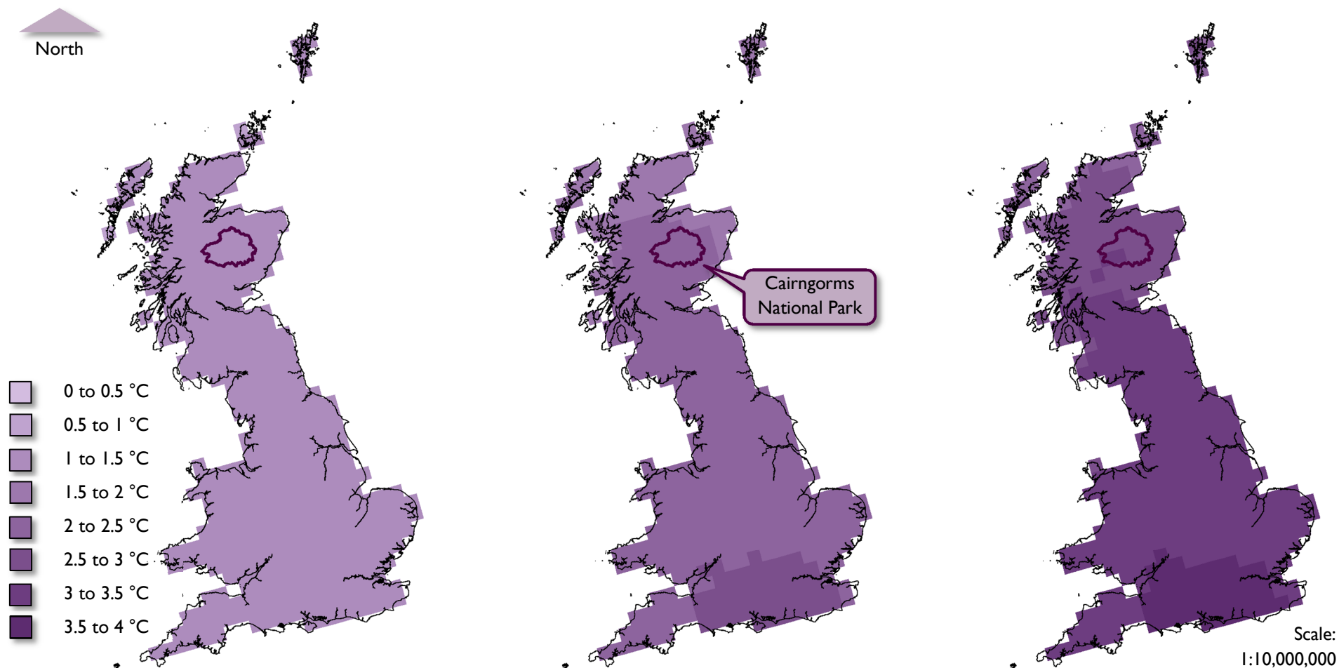
Figure 17 Mean annual temperature increase 2020s. Medium emissions scenario, central estimate.
