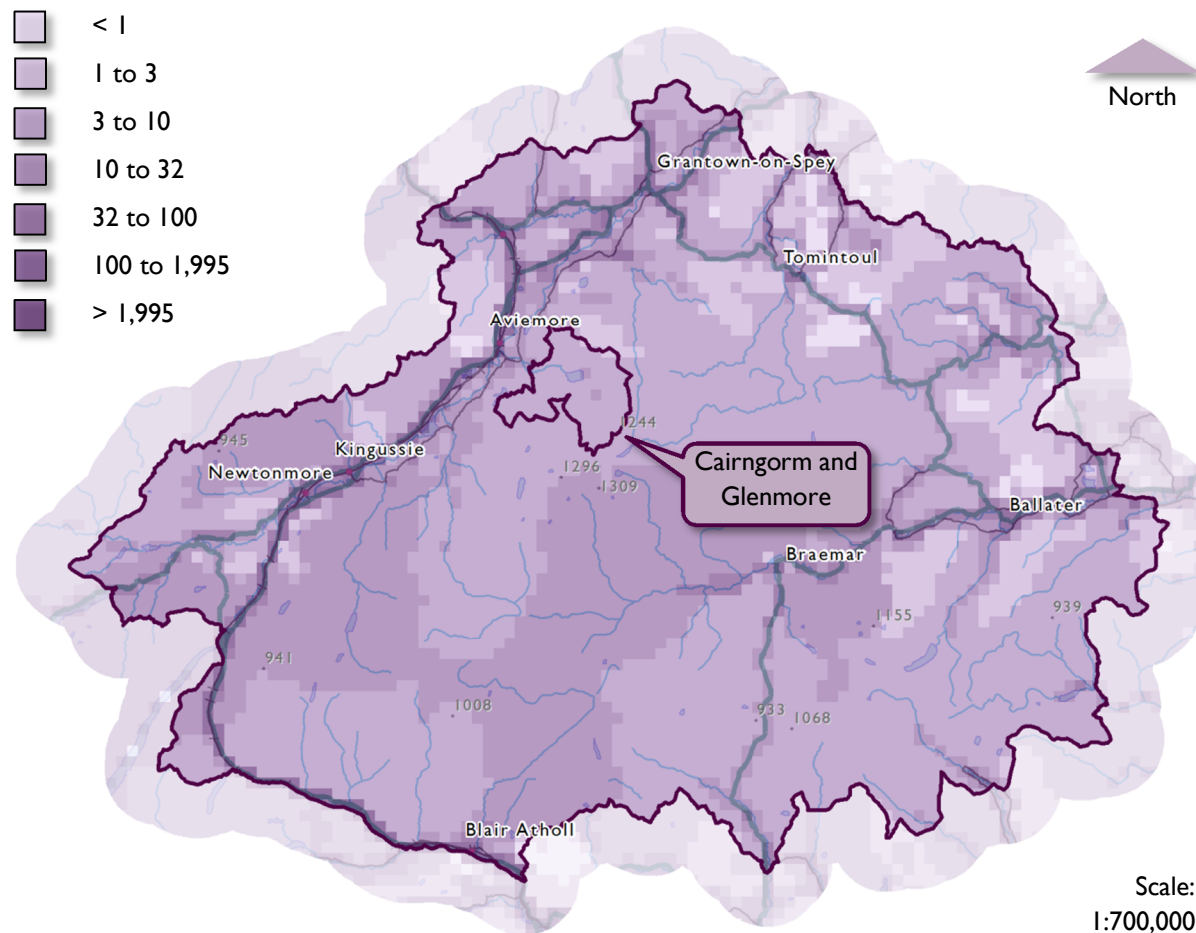
Figure 20 Carbon Dioxide (as Carbon) Emissions in tonnes for the Cairngorms National Park in 2012.
