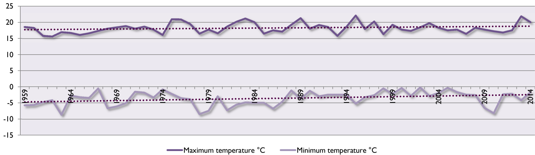
Figure 12 Maximum and minimum annual temperatures at Braemar Weather Station (Met Office, 2015).
