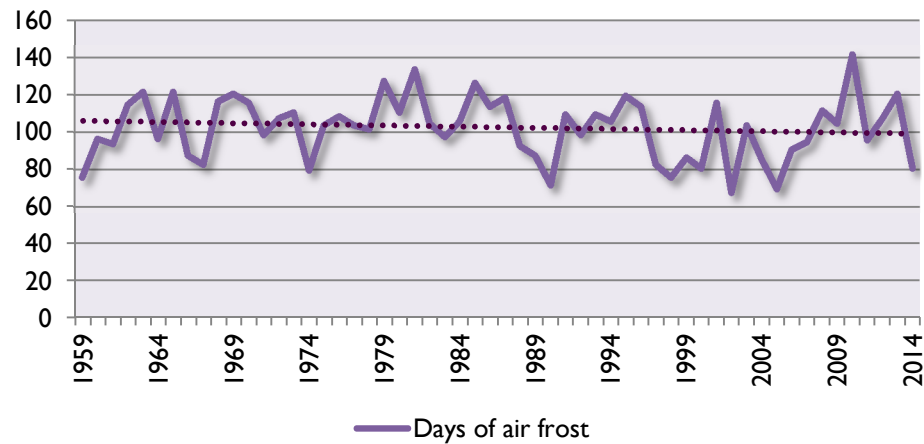
Figure 13 Days of frost at Braemar Weather Station (Met Office, 2015).
