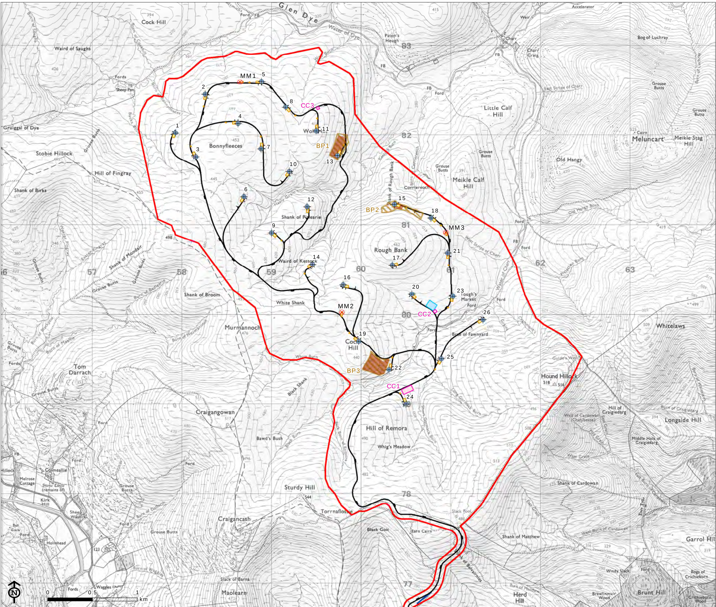
Figure 2a: Proposed Site Layout
