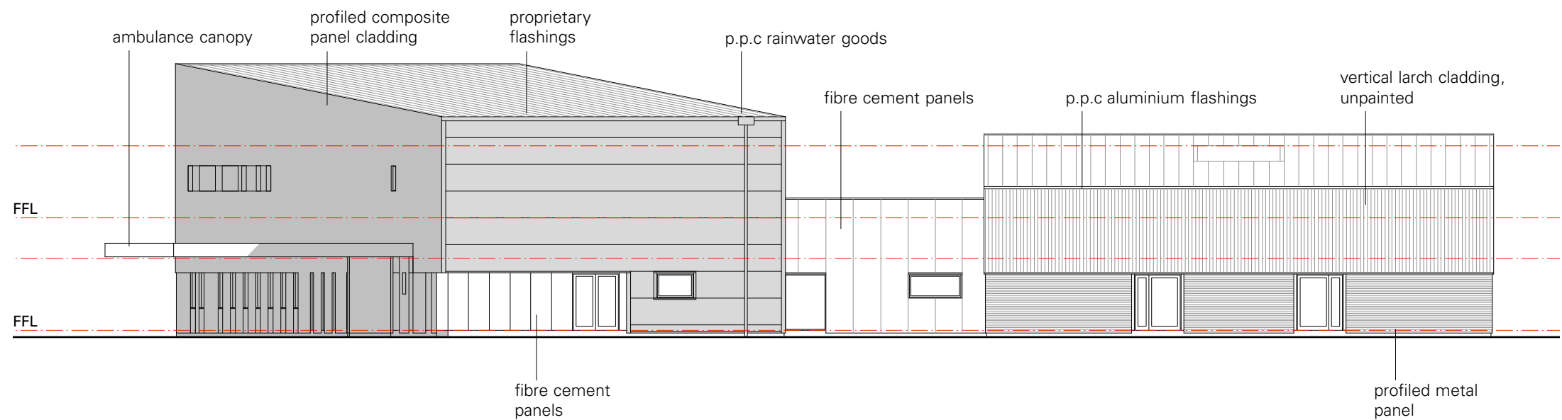
South Elevation
