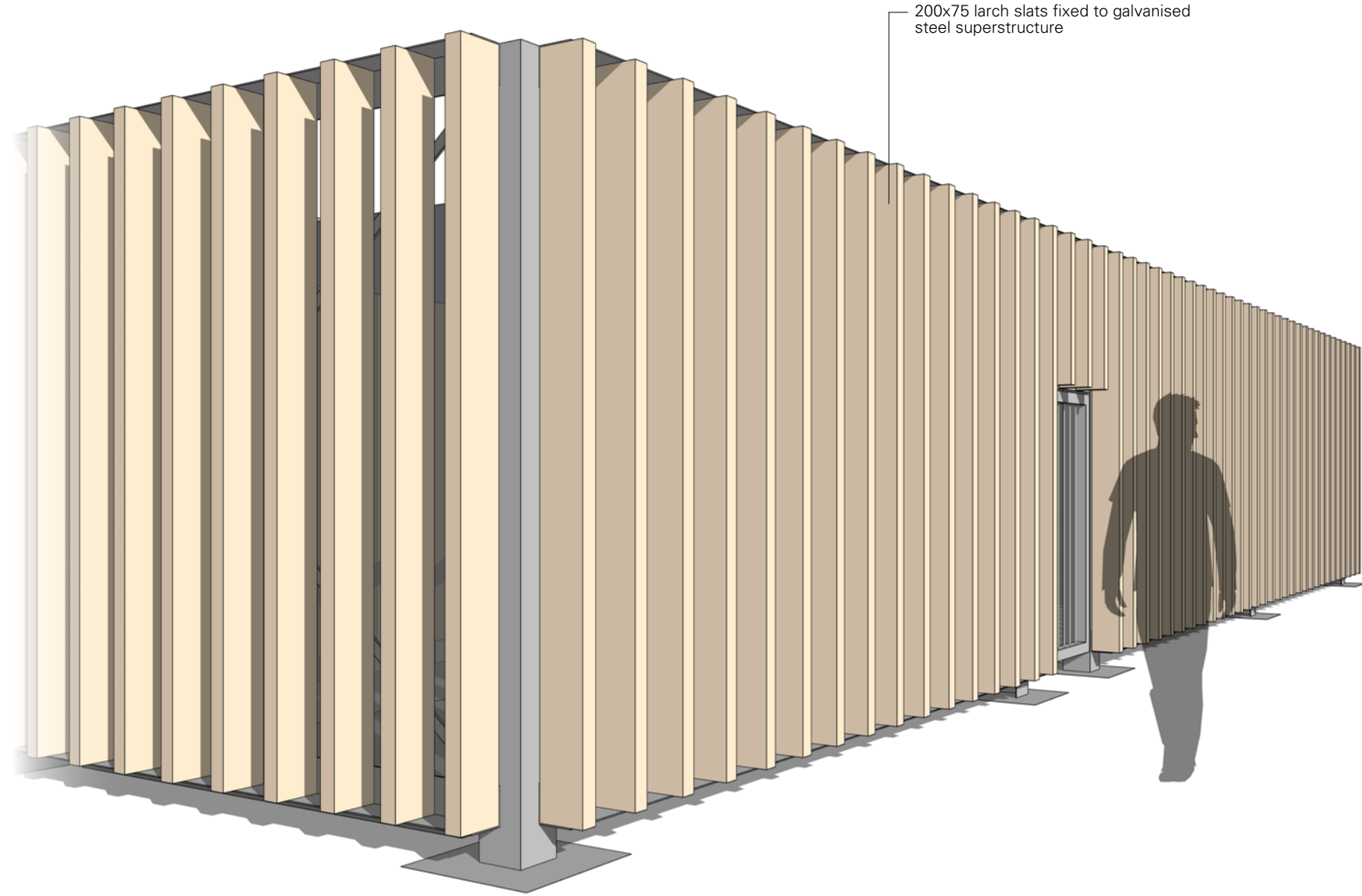
Indicative illustration of typical corner
