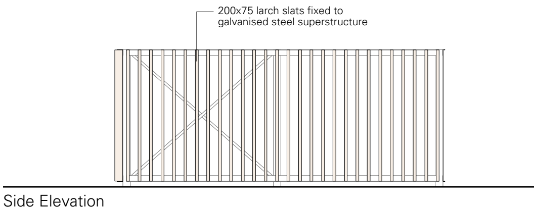
Side Elevation
