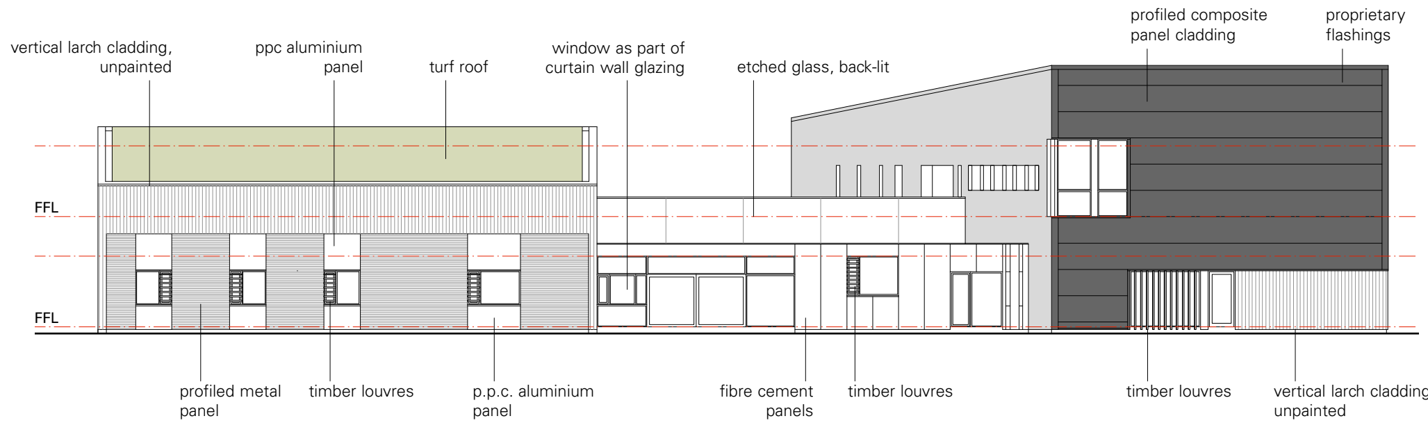
North Elevation
